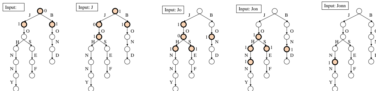
Figure 6: Illustrating Algorithm 5.1
