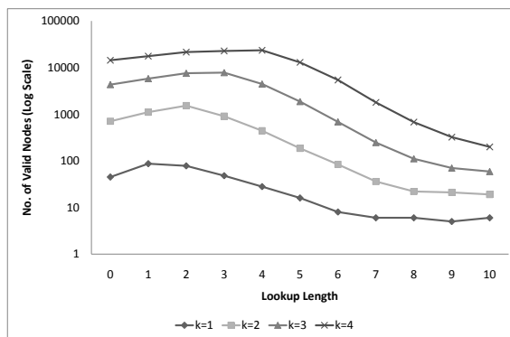
Figure 7: Valid Nodes (log scale) Vs. Lookup Lengths and Edit Distance Thresholds
