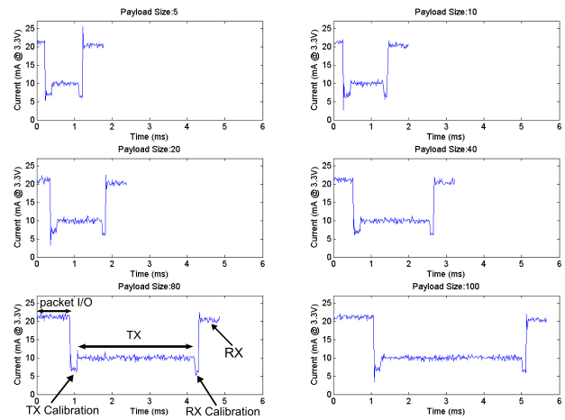
Figure 3. The 802.15.4 current vs. payload.
