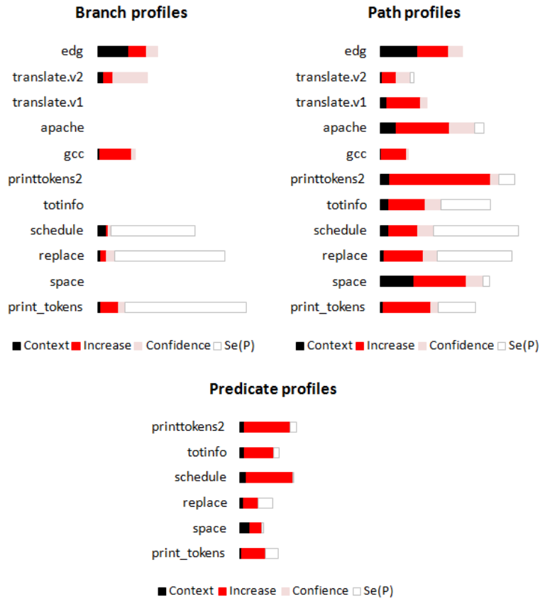
Figure 5: Bug thermometers used to visualize information about predictors. The figure shows the average context, the increase, the confidence in increase and the number of times the predictor is executed in successful runs for branch and path predictors.
