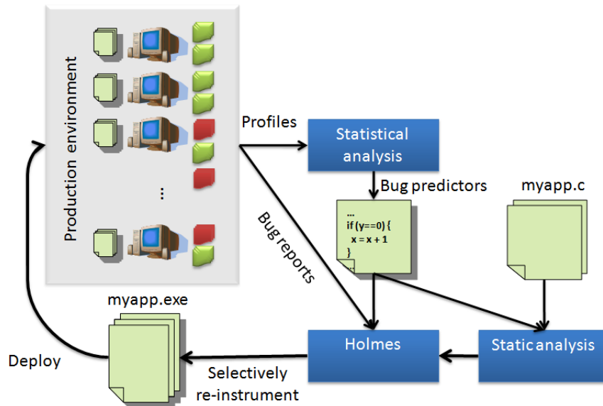
Figure 2: The HOLMES framework.
