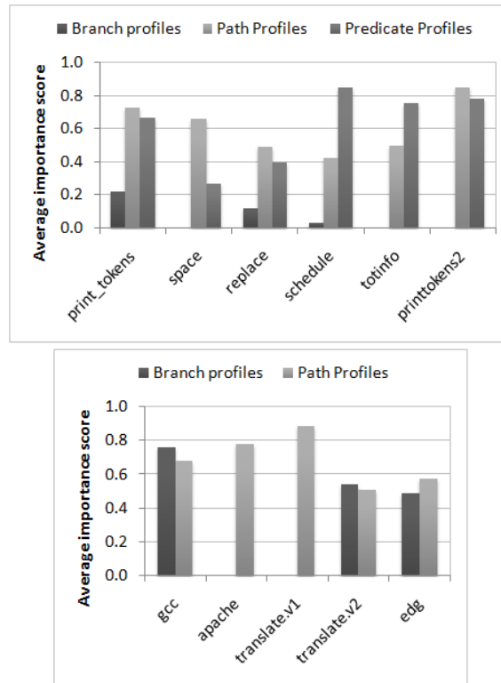
Figure 4: Average importance scores assigned to bug predictors for various profiling schemes. High scores are better.
