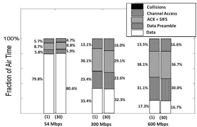
Figure 16: WiFi-Nano overheads
