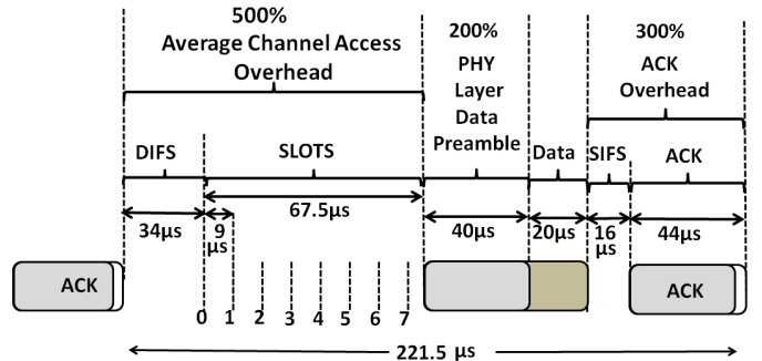
Figure 1: Overheads in 802.11 at 600 Mbps
