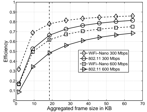
Figure 18: Frame Aggregation
