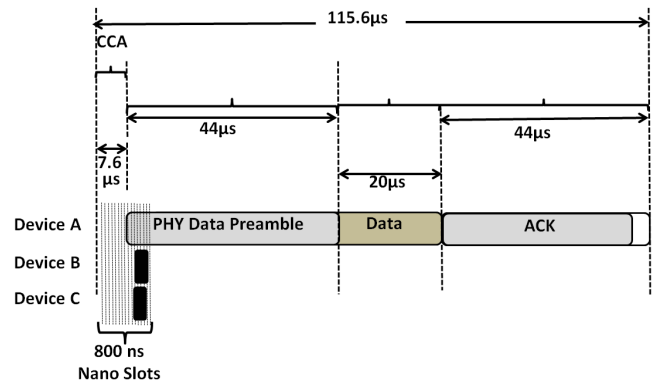
Figure 3: WiFiNano transmissions at 600Mbps
