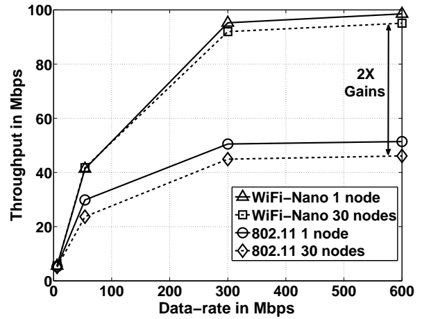
Figure 15: Throughput
