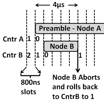
Figure 4: Making slot duration independent of carrier sensing time
