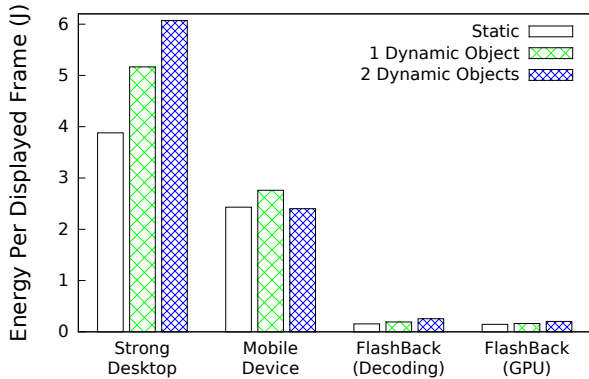
Figure 11: FLASHBACK significantly reduces the energy consumed per frame displayed even when a frame must be decoded first. Desktop measurements were conducted on a different, less energy-efficient machine.
