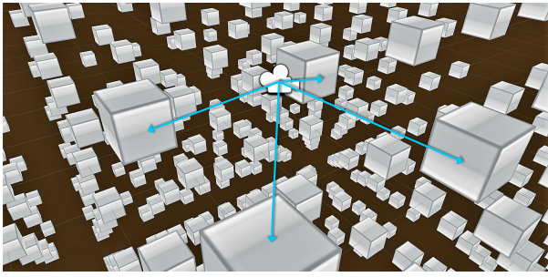
Figure 3: Logical layout of megaframes. Each cube represents a megaframe’s cache index visualized in 3D space. Arrows depict the distance from the closest few megaframes to the current pose query, represented by the camera icon.
