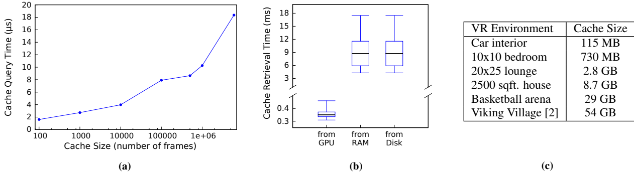
Figure 12: (a) Cache query time scales well with the size of the cache, allowing FLASHBACK to performantly support very large caches. (b) Performance when retrieving 4k megaframes from all three cache levels. The y-axis break shows very small retrieval times from GPU. (c) Cache size on Flash storage (uncompressed) for various static virtual environments.
