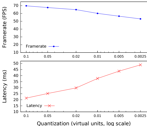
Figure 15: The effects of quantization (cache density) on FLASHBACK’s performance: framerate and latency.
