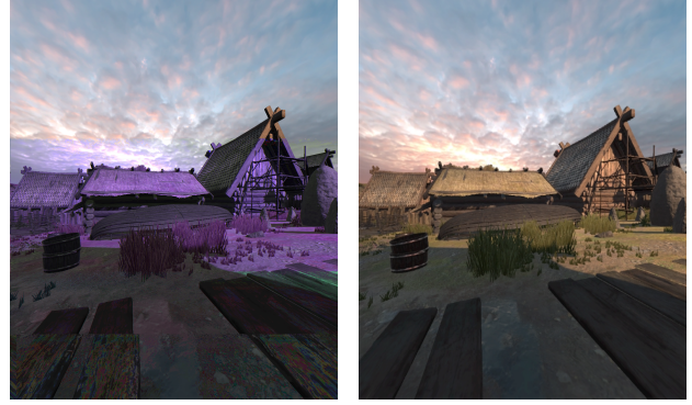
Figure 10: Sample frames outputted at the same trace pose (post-alignment), used as SSIM inputs. The left frame is the pristine image ( f^* ) from stock Viking Village. The right frame ( f ) represents a worst-case GPU cache miss in FLASHBACK, demonstrating the quality of our graphical warp.
