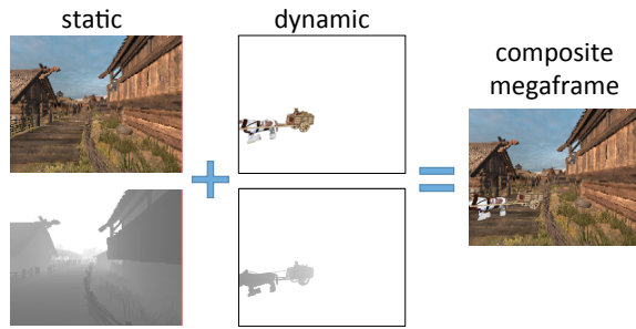
Figure 6: Compositing Dynamic Objects With Static Scenes. Croppings of the megaframes (a single cube face) for one static scene and one dynamic object are shown.
