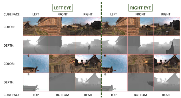
Figure 2: Each cache entry contains a megaframe. The twenty-four faces of the megaframe represent the left and right eye cube maps for RGB color and depth.
