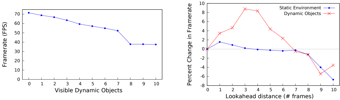
Figure 13: FLASHBACK scales well to a moderate number of visible dynamic objects, maintaining a high framerate until insufficient memory causes page thrashing.
