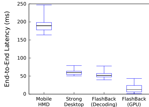
Figure 8: FLASHBACK achieves an end-to-end latency up to 15X shorter than a weak mobile device rendering locally, with worst-case latency no higher than that of a gaming desktop.
