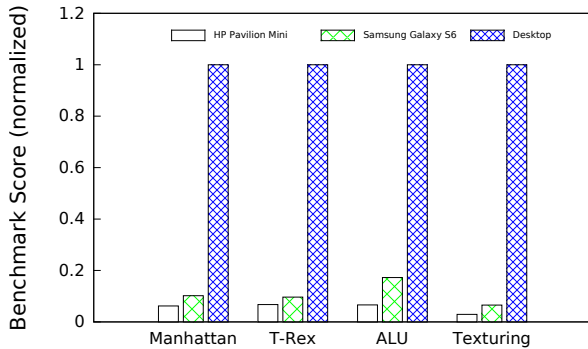
Figure 7: Four GFXBench benchmarks across three devices demonstrate that the HP Pavilion Mini is less capable than a Galaxy S6, and that both devices are an order of magnitude weaker than a VR-capable desktop [1].
