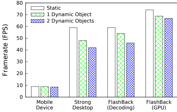
Figure 9: FLASHBACK delivers framerates up to 8X higher than a mobile HMD rendering locally.
