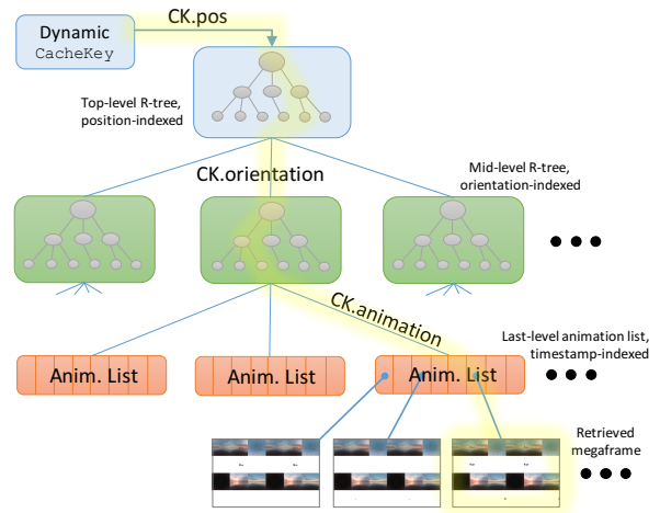
Figure 5: Nested R-Trees for Retrieval of Dynamic Objects. Dynamic objects are indexed by relative position (top-level R-tree), orientation (nested R-trees), and animation stages (simple lists).
