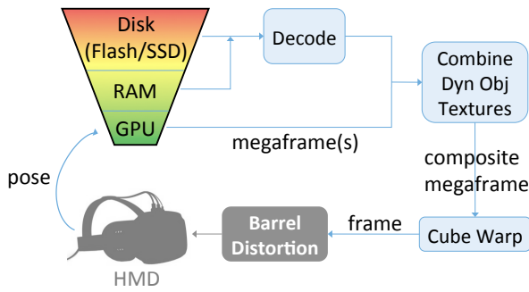
Figure 1: FLASHBACK runtime operation. FLASHBACK uses the HMD pose to query the cache and decode the retrieved megaframe if necessary, then it combines that static megaframe with any dynamic object megaframes, and finally warps the megaframe into a single final frame for the HMD.
