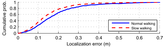
Figure 9: Cumulative distribution of localization error: The median error is 0.16m for normal walking and 0.13m for slow walking. 95% of errors are under 0.36m (slow walking) and 0.47m (normal walking).
