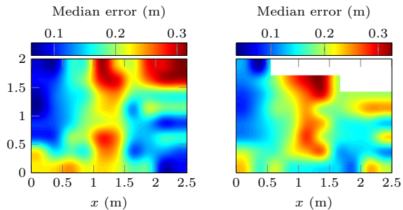
Figure 8: Median localization error over the covered area, without any object present (left) and with a grounded metallic cart in the top right corner (right). Because the cart was in the way, no trajectories entered the white zone. In both maps, the median error is largest at the border between the two cells ( x = 1.25 m).
