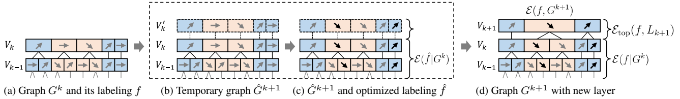
Figure 3. Bottom-up Graph Construction (one step). Each rectangular cell in the illustration represents a node i \in V_l and a set of contiguous cells represents a graph layer V_l . The arrows and colors denote flow and alpha labels f_i (red: foreground, blue: background). (a) Graph G^k and its labeling f . (b) By duplicating the top layer V_k of G^k , we create a temporary graph \hat{G}^{k+1} as an approximation of G^{k+1} . (c) We optimize the labeling \hat{f} on \hat{G}^{k+1} . The number of unique labels in V_k' is reduced by label costs [15] to induce region merging. (d) V_k' is converted into a new layer V_{k+1} , by merging nodes of V_k' assigned the same label that form connected components in \hat{G}^{k+1} .
