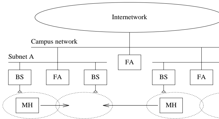
Figure 1: Hierarchical organization of a wireless internet network, including wired links, wireless cells, base stations, and mobile hosts.
