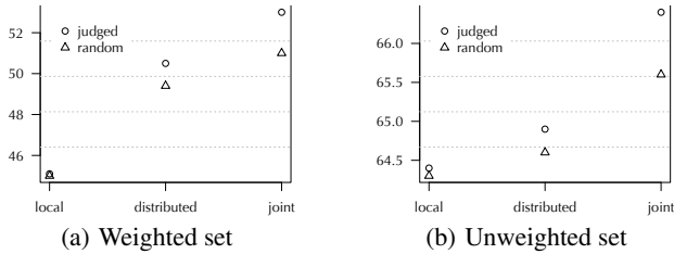
Figure 4: The duet model demonstrates significantly better NDCG performance ( p < 0.05 ) on both test sets when trained with judged non-relevant documents as the negative examples, instead of randomly sampling them from the document corpus. The distributed model also shows statistically significant NDCG gain ( p < 0.05 ) on the weighted set, and a non-statistically significant NDCG gain on the unweighted set.
