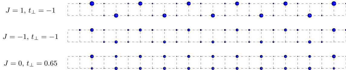
FIG. 6. Strength of the density correlation functions \langle n_{0,\uparrow} n_{j,\uparrow} \rangle and \langle n_{0,\downarrow} n_{j,\downarrow} \rangle (shown only with j > 0 ) for values of the parameters representative of the three different phases at quarter filling. The diameters of the blue, filled dots are proportional to the strength of the correlation; the upper row in each panel corresponds to \langle n_{0,\uparrow} n_{j,\uparrow} \rangle , while the lower row corresponds to \langle n_{0,\downarrow} n_{j,\downarrow} \rangle , and the distance from the left end indicates j .
