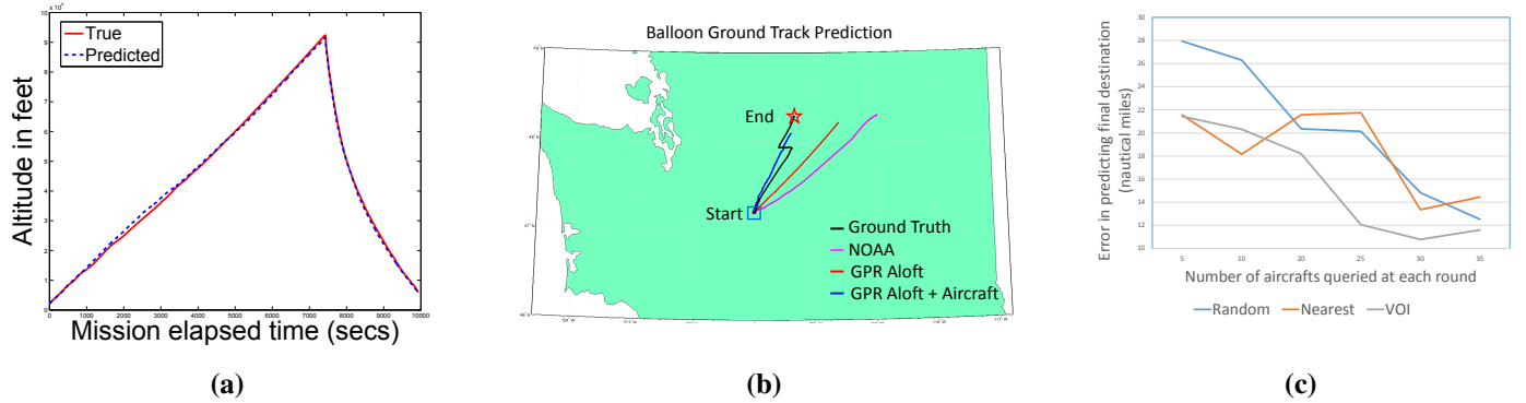
Fig. 6. (a) This figure demonstrates the accuracy in determining the ascent profile of the second balloon. (b) The path predicted using the three wind estimation models. The proposed model (blue) estimates the path far more accurately than the NOAA forecasts (magenta) and the GP aloft model (red) based only on the wind stations data. (c) Performance comparison of the VOI-based querying of aircraft data with random sampling and the nearest heuristic. The figure shows that significant accuracy in path prediction can be obtained for a fraction of cost if the decision-theoretic method proposed in the paper is used.
