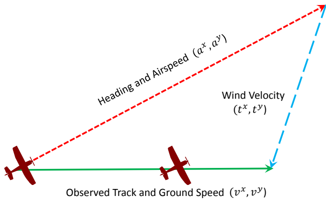
Fig. 3. Graphical representation of the wind triangle. The aircraft maintains an assigned heading at a reported constant and known airspeed (a^x, a^y) , while the observed wind (t^x, t^y) changes the observed course and the ground speed (v^x, v^y) via a vector addition. We use a Cartesian representation for velocities where the x and the y components denote projection of the vector on easterly and northerly headings respectively.
