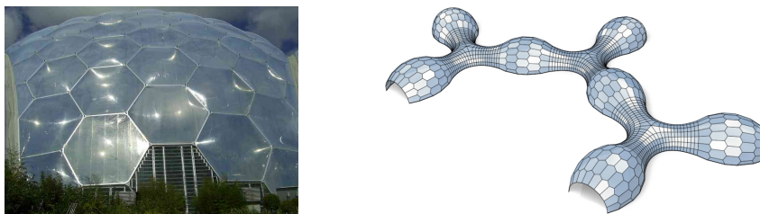
FIG. 1. Left: A geodesic dome constructed using a P-Hex mesh in the Eden Project in UK; right: the convex parts of this model are constant mean curvature (CMC) surfaces modeled by P-Hex meshes [6].
