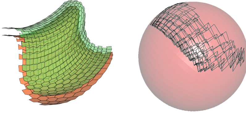
FIG. 10. Left: A free-form P-Hex mesh and its constant face-distance offset mesh; right: the Gauss image of the P-Hex mesh, whose faces are tangent to the sphere S^2 .
