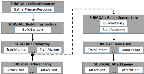
Figure 2: A tactical plan (left) with a contingent branch (right).
