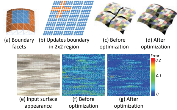
Figure 6: Whole surface mapping. (a) For each patch, we fix its central part (shown in blue) and only update the height and BRDF weights of the patch boundaries (shown in brown) by global optimization. (b) In each step, we update the height and BRDF weights of 2 \times 2 patch boundaries (shown in red). For the input appearance shown in (e), (f) and (g) show the error maps of the bi-scale mapping result before and after the whole surface mapping, the patch boundaries before and after optimization are also illustrated in (c) and (d).
