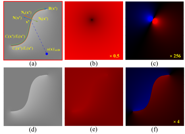
Figure 2: A diffusion curve texture defined by two control curves: an S-shaped curve, and a curve along the image boundary. (a) Control curves with boundary conditions (0.75 for the right S-shaped boundary, 0.5 for the left S-shaped boundary and the image boundaries). (b) Profile of Green's function kernel G(\mathbf{x}, \mathbf{x}') from one point on a control curve. (c) Profile of Green's function kernel G_n(\mathbf{x}, \mathbf{x}') from one point on a control curve. (d) Diffusion curve image computed from all of the Green's function kernels. (e) Image generated from only the Green's function kernels G(\mathbf{x}, \mathbf{x}') . (f) Image generated from only the Green's function kernels G_n(\mathbf{x}, \mathbf{x}') . In the rightmost two columns, red indicates positive values, while blue indicates negative values.
