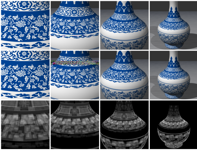
Figure 7: Rendering for zoomed-out views. The top row is rendered with our diffusion curve texture. The middle row is rendered with a rasterized texture of resolution 8192 \times 8192 , which generates results similar to our method. The bottom row shows the sampling rates with our method. Our rendering times are 74 ms, 76 ms, 82 ms, and 88 ms from left to right.
