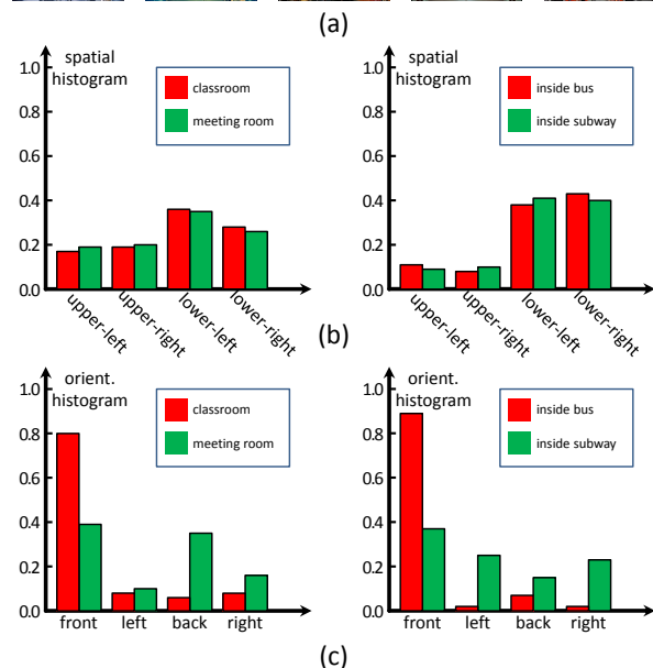
Figure 1. (a) Sample images for 4 scene categories from the MIT Indoor-67 dataset [32]: classroom , meeting room , inside bus and inside subway (from top to bottom). For both category pairs, the orientational features are more discriminative than the spatial features. (b) The spatial distributions of chairs in both confusing pairs are very similar. (c) The orientational distribution of chairs are much more dispersive.
