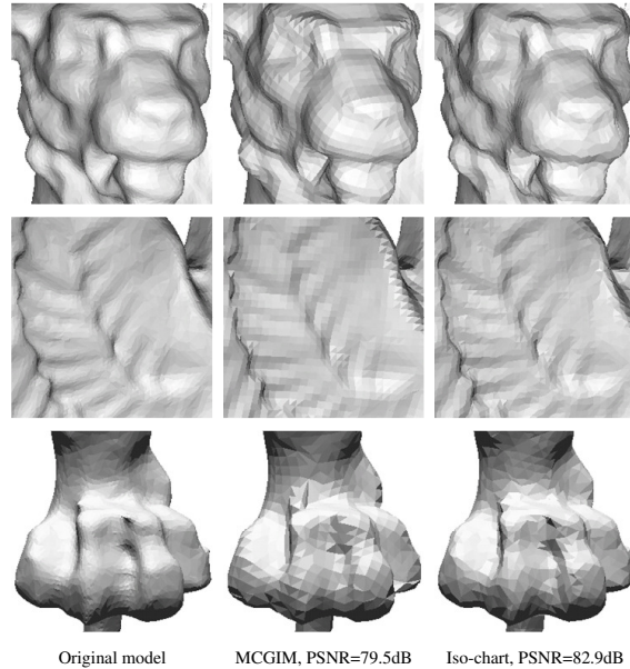
Figure 7: Comparison of geometry remeshing methods. Geometry images have resolution 256 \times 256 .
