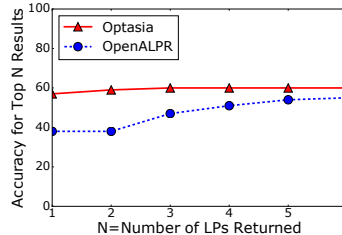
Figure 8: LPR Accuracy for Top N results.
